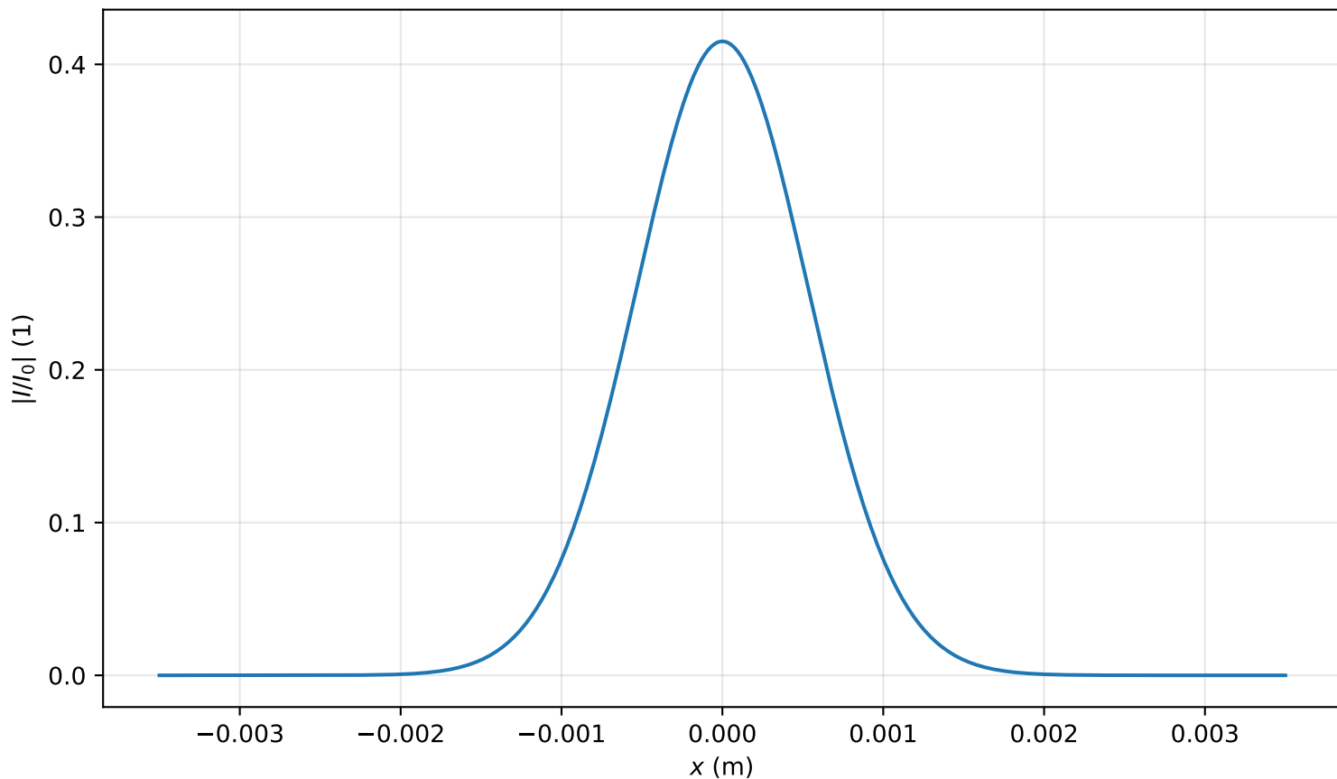
Intensity profile I(x, y = 0, z = 2.548m)/I_0 , P_{in}=0.1P_{cr} , artificial time
